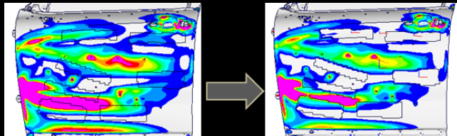
Door panel deformation
