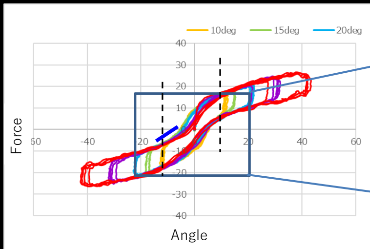
Steering Angle VS Operation Force
